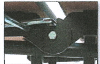
Locks: Unique dual-purpose lock holds table securely in both up and down position. It is easily reached from both sides of the table.
